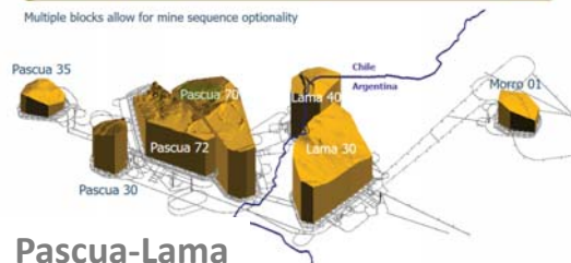
Preliminary Block Cave Mine Layout
