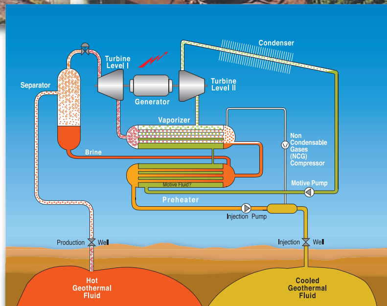
Two-Phase Binary Geothermal Power Plants
