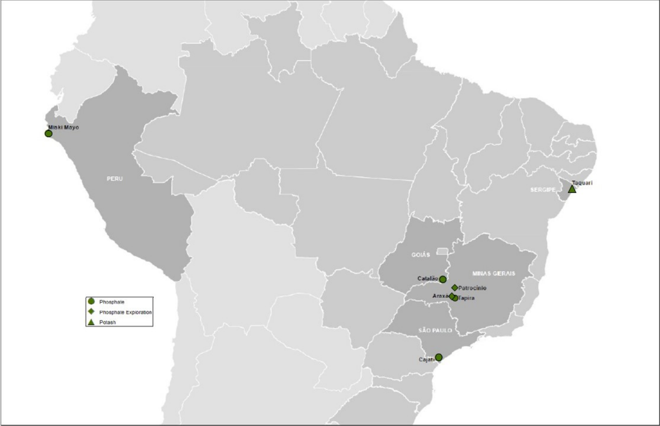
Figure 2.2: South America Resource and Reserve Location Map
